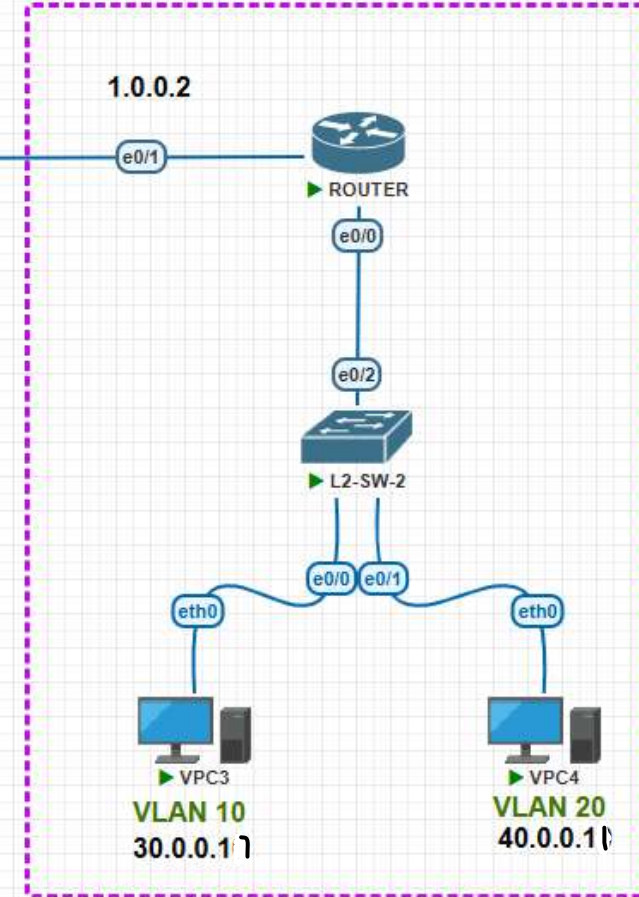
ROUTER ON-A-STICK
